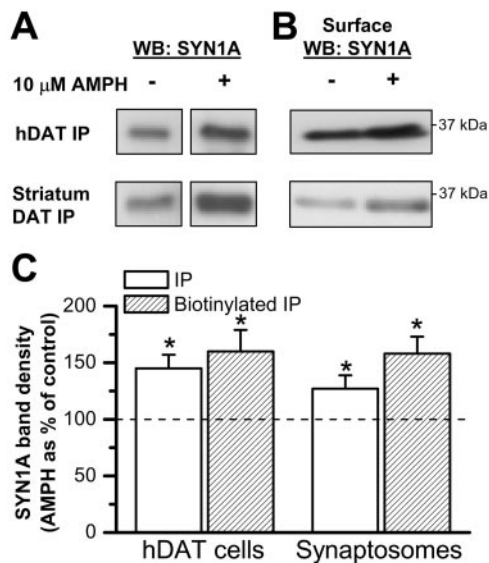
Fig. 2. AMPH promotes DAT/SYN1A association. A, hDAT cells transfected with SYN1A or mouse synaptosomes were treated with 10 \mu M AMPH for 5 min at 37°C. DAT proteins were immunoprecipitated and immunoblotted for SYN1A. B, surface fractions were isolated by biotinylation. DAT proteins were immunoprecipitated and immunoblotted for SYN1A. C, the immunoprecipitated band densities were quantified, normalized to the corresponding density of total SYN1A (data not shown), and expressed as a percentage of vehicle control ( n = 3-7 ; *, p < 0.05 , Student's t test).
