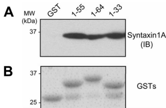
Fig. 1. SYN1A directly interacts with hDAT. A, GST pull-down experiments confirm a direct interaction between SYN1A and hDAT and demonstrate that the hDAT N terminus mediates this interaction. Purified SYN1A \Delta\text{TM} was incubated with GST alone or with GST-hDAT N-terminal fusion proteins composed of the indicated residue numbers. The samples were then immunoblotted for SYN1A. Each of the three fusion proteins tested showed a signal for SYN1A but no signal was observed for GST alone. The experiment displayed is representative of five experiments. B, an SDS-polyacrylamide gel electrophoresis gel of the GST fusion proteins used in A stained with GelCode Blue demonstrating fusion proteins of the correct size with minimal degradation.
